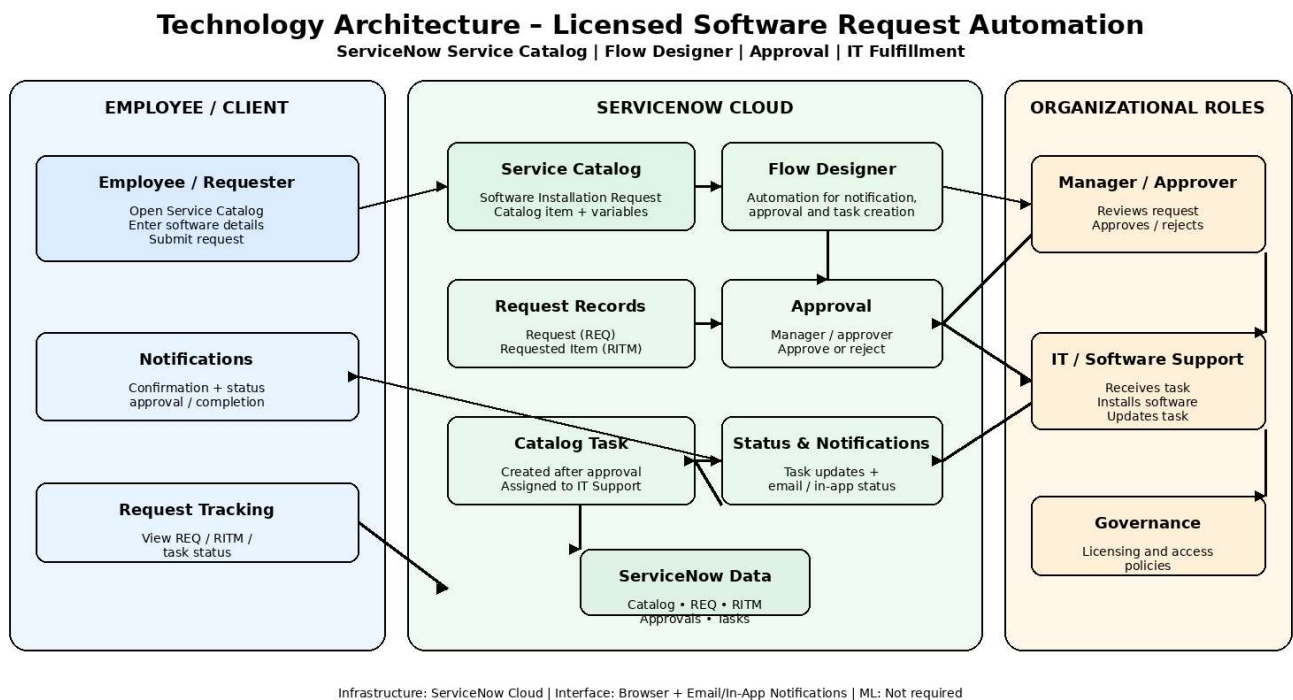
Figure 1: Technology Architecture for Licensed Software Request Automation
